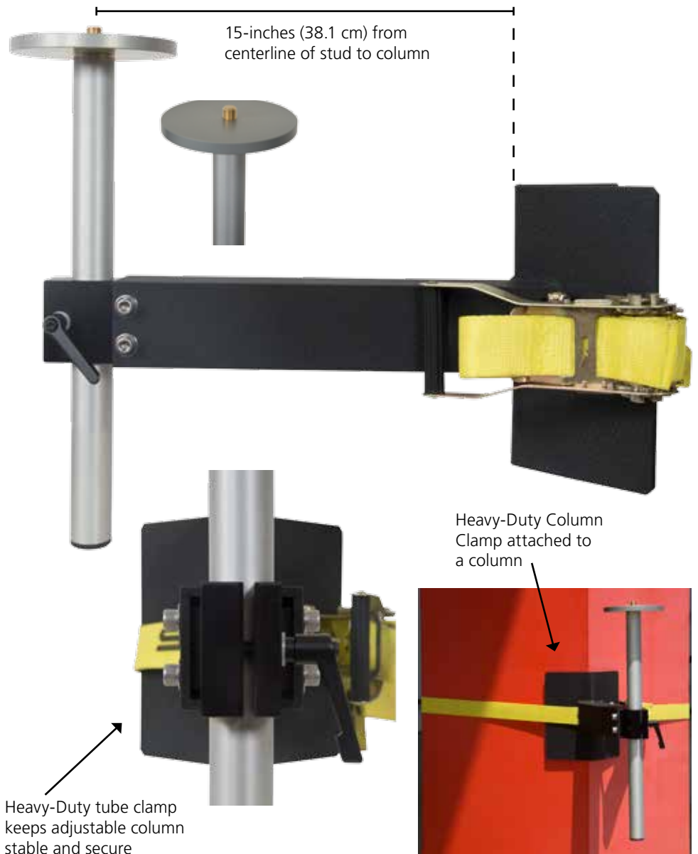
4852-16 Heavy-Duty Column Clamp
